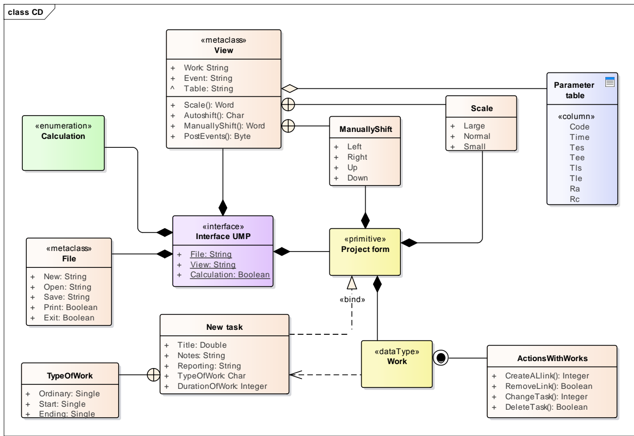
Fig. 6. Class Diagram
