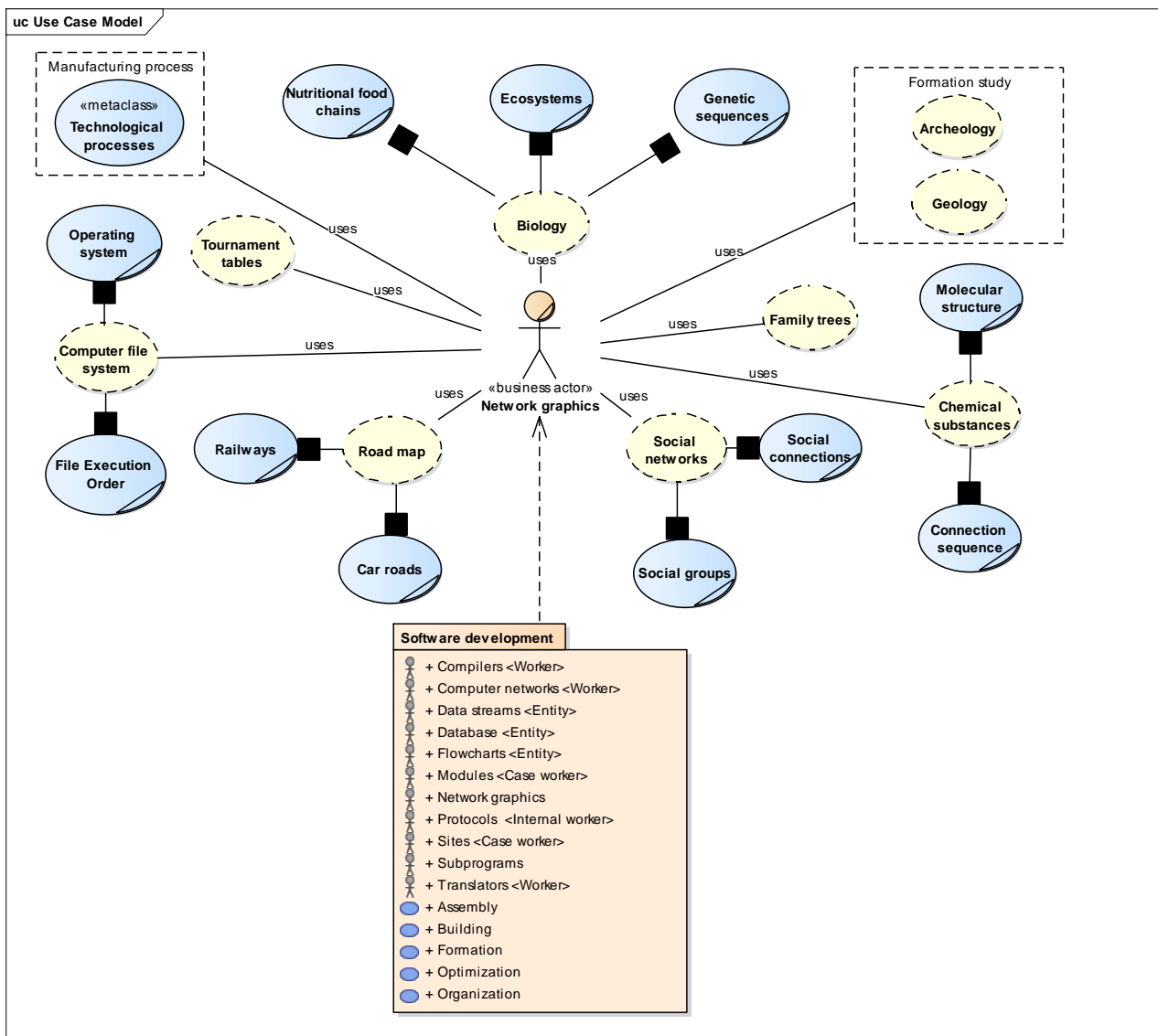
Fig. 1. Use-Case Diagram
