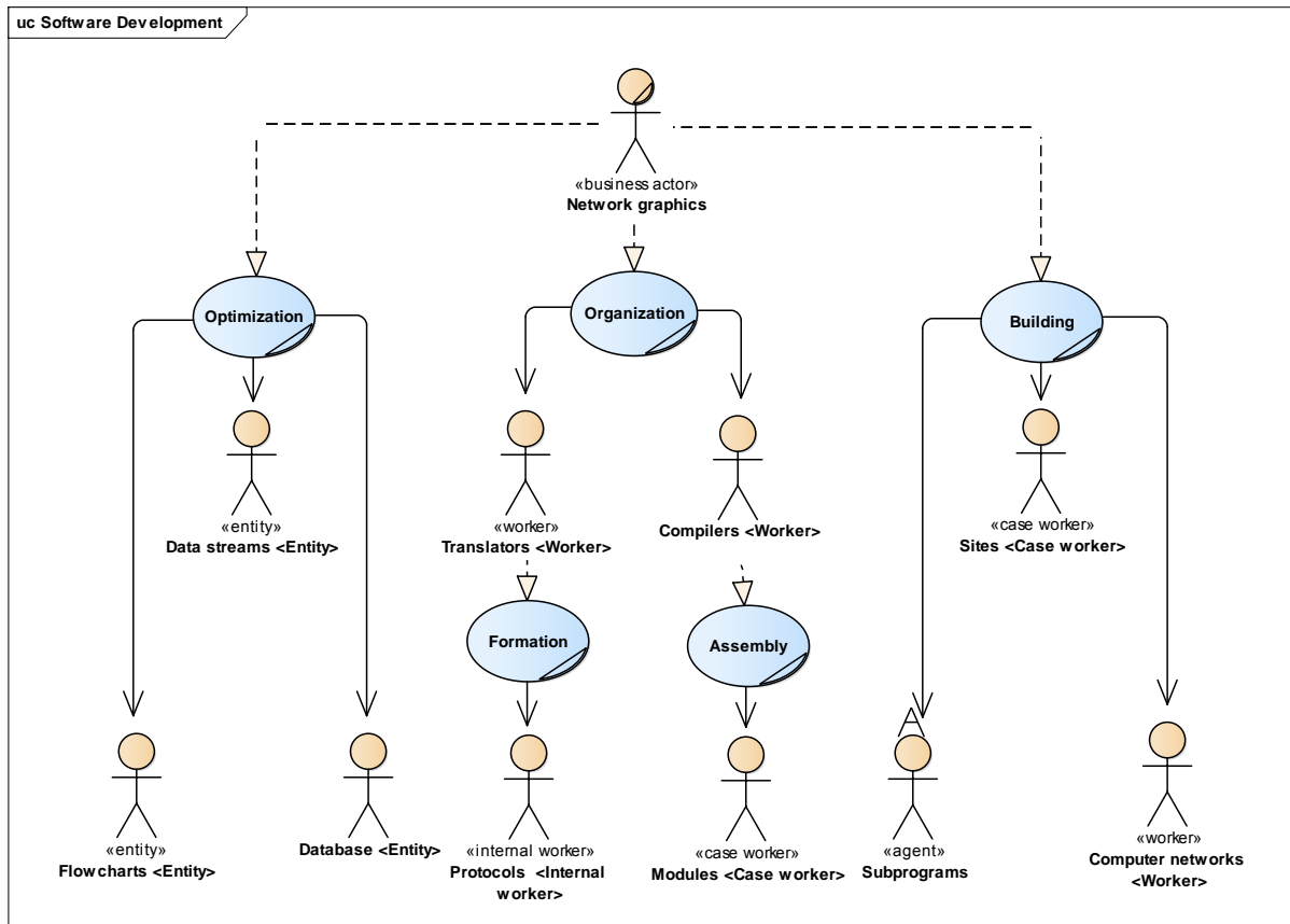
Fig. 2. Diagram-Package “Software Development”
