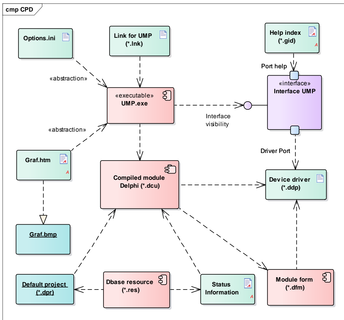
Fig. 7. Component Diagram
