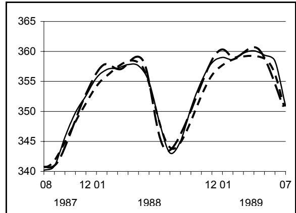
Fig. 5. Concentration of atmospheric CO 2 (ppm) at Barrow since August 1987 till July 1989 (solid line – observations, short dotted line – weak EP pattern indices, long dotted line – strong EP pattern indices).
