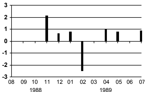
Fig. 4. EP pattern indices since August 1988 till July 1989.
